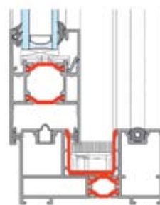
Double Track
