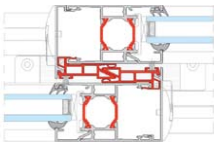
Interlock Detail
