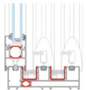
Triple Track
